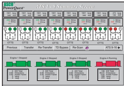
Fig. 23: ASCO PowerQuest® Vpi 32.15
